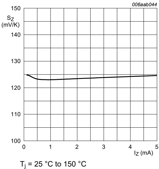
Fig. 3. Temperature coefficient as a function of working current; typical values
