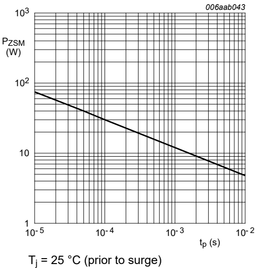
Fig. 2. Non-repetitive peak reverse power dissipation as a function of pulse duration; maximum values
