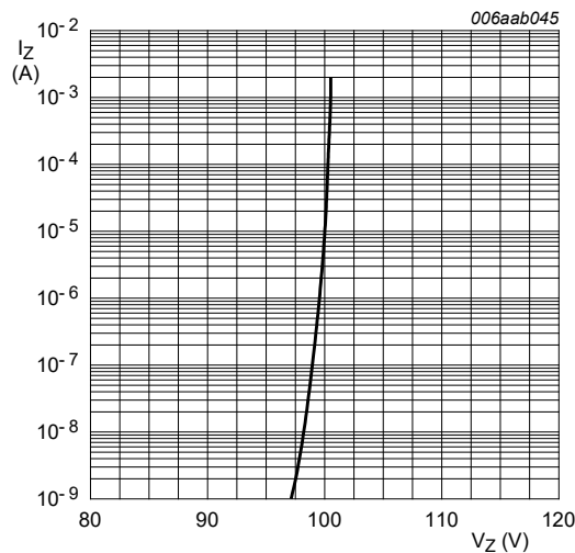
Fig. 4. Working current as a function of working voltage; typical values
